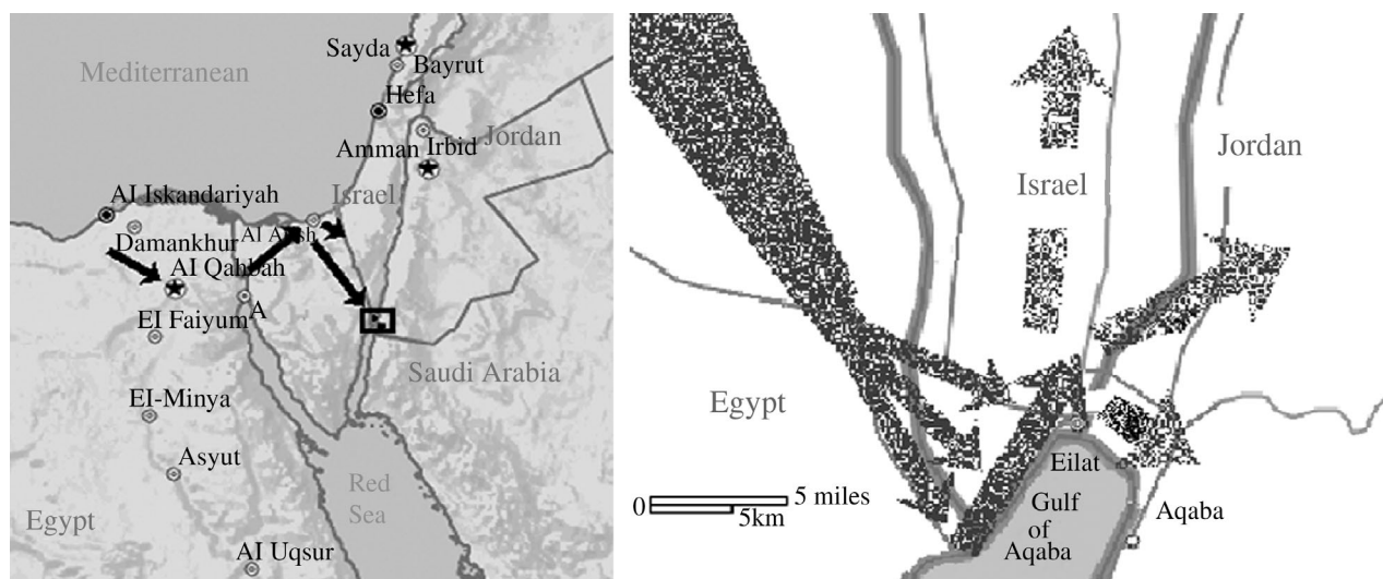
Figure 1. Trajectories of locust swarms near the Gulf of Aqaba. Swarms of migrating desert locusts reached the northern Gulf of Aqaba from the Sinai peninsula on 21–23 November 2004, turned north when reaching the water, and crossed to Jordan, just over the northern coast of the gulf. Modified with permission from Haaretz news service.
